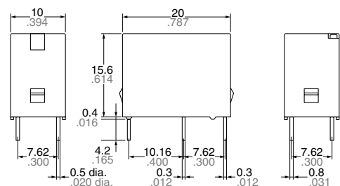
1 Form C
