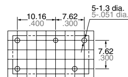
1 Form C
