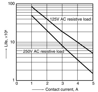
2. Life curve
